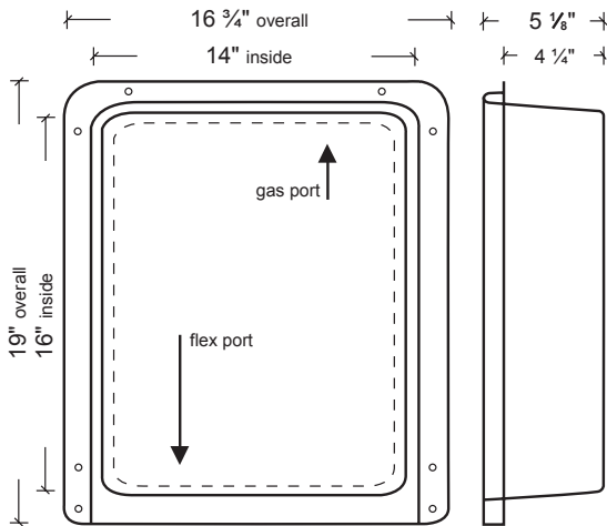
Recessed Dryer Vent Box MODEL 4D
