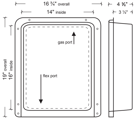
Recessed Dryer Vent Box MODEL 3D
