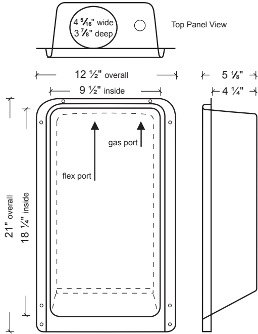
Recessed Dryer Vent Box MODEL 425
