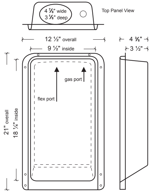
Recessed Dryer Vent Box MODEL 350
