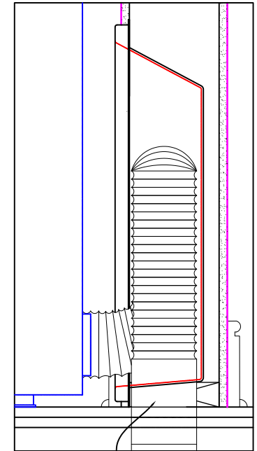
STAND-ALONE
