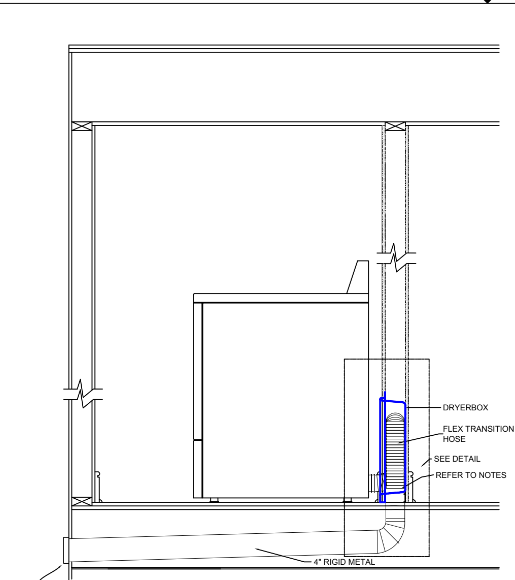
Model 466 Dryerjack (optional) www.dryerwallvent.com
