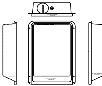
Sectional View
